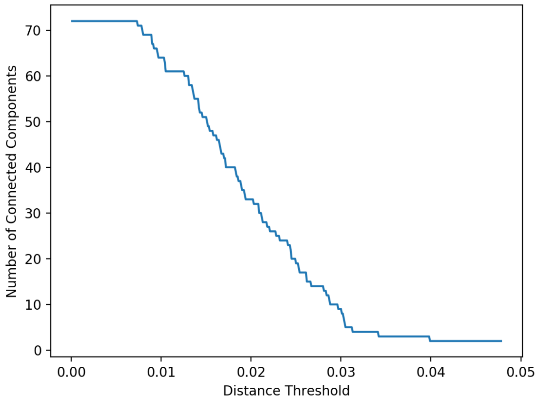
Figure IV.2: Distance threshold versus number of connected components
